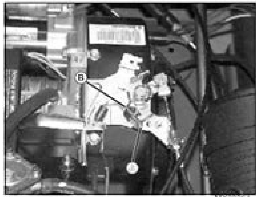
Throttle adjustment lever cover removed for photo clarity. Governed low idle adjustment can be made with cover on.
