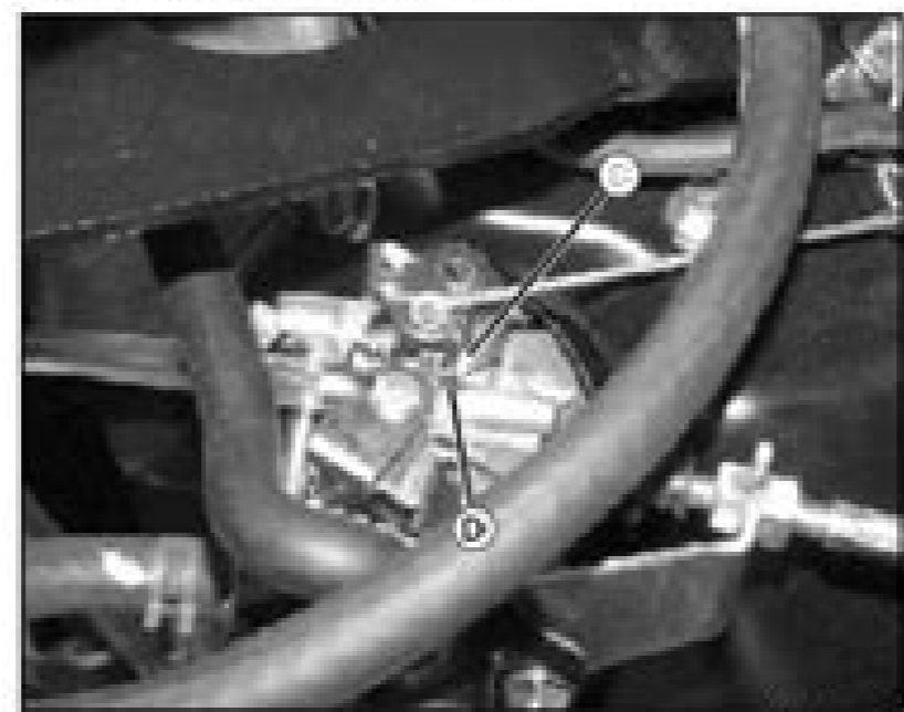
Travel is limited to about 3/4 turn on idle mixture screw for emission compliance. Do not force screw beyond limit tabs, screw is designed to break off if forced.
